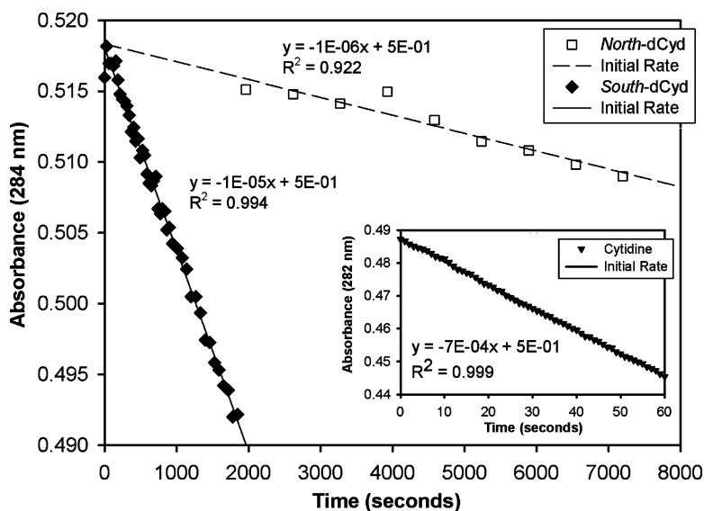
FIGURE 5 Initial time course data for the CDA (900 nM) catalyzed deamination of North -dCyd ( \square ) and South -dCyd ( \blacklozenge ) followed at 284 nm ( \Delta\epsilon^{284} = -5000 ). The inset shows initial time course data for the catalyzed deamination of the natural substrate cytidine ( \blacktriangledown ) by CDA (0.9 nM) monitored at 282 nm ( \Delta\epsilon^{282} = -3600 ).
