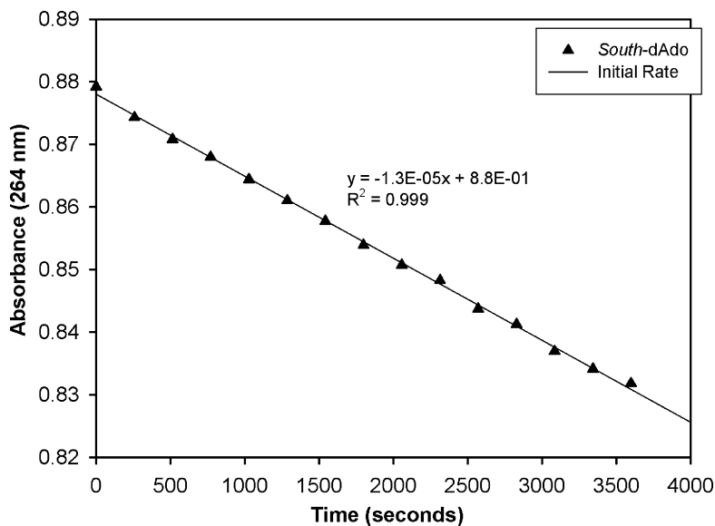
FIGURE 1S Initial rate for the ADA (bovine spleen) catalyzed deamination of South -dAdo (▲) at 60 \mu M and 25°C.
