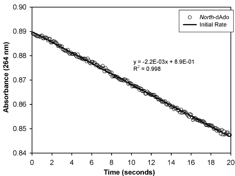
FIGURE 2S Initial rate for the ADA (bovine spleen) catalyzed deamination of North -dAdo (○) at 60 \mu M and 25°C.
