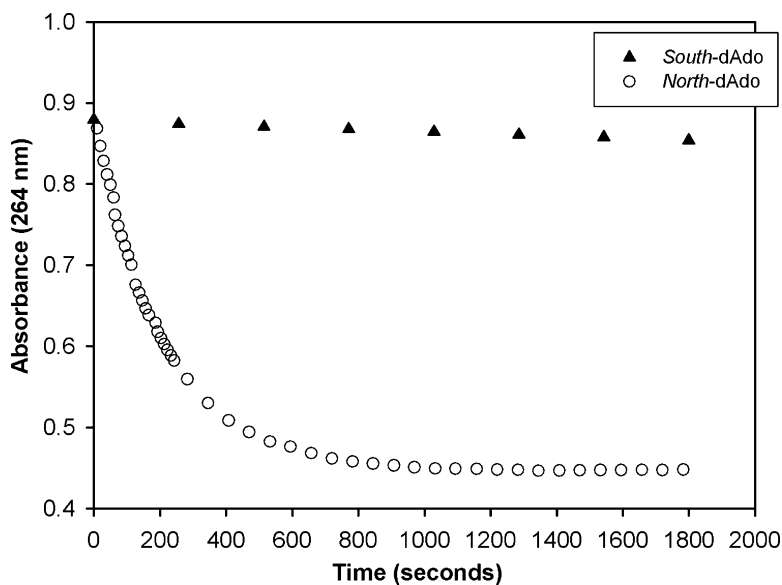
FIGURE 3 Bovine spleen ADA ( \sim 0.5 units) deamination of South -dAdo ( \blacktriangle ) and North -dAdo ( \circ ) at 60 \mu\text{M} determined by measuring the decrease in absorbance at 264 \text{ nm} ( 25^\circ\text{C} ).
