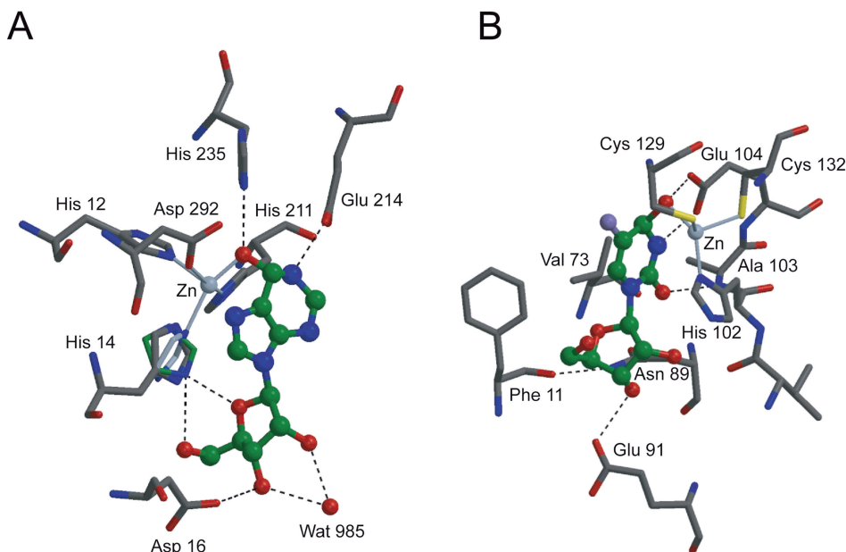
FIGURE 2 (A) Bovine ADA in complex with hydrated nebularine. [11] Ligand is shown in ball-and-stick representation, with green carbons. The crystal coordinates of residue His 14 are shown in dark gray. This conformation is suggested to be an average of two rotamers: one (in green) where the N \delta atom makes a bifurcated hydrogen bond to the sugar moiety in the ligand, and one (in light blue-gray) where the zinc atom lies in the plane of the imidazole ring. (B) E. coli CDA in complex with hydrated 5F-zebularine. [13]
