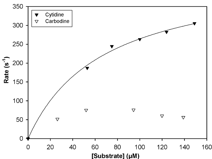
FIGURE 6 Michaelis-Menten plot for enzyme catalyzed deamination of cytidine ( \blacktriangledown ) and carbodine ( \nabla ). The solid line represents a non-linear regression fit of the cytidine data to the Michaelis-Menten equation.
