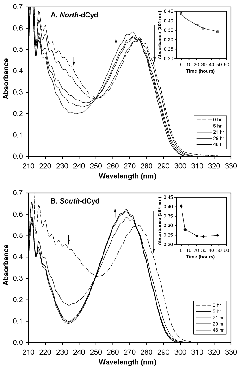
FIGURE 4 Full UV spectrum for the enzymatic deamination of North - and South -dCyd over time. A clean isobestic point at 250 nm is maintained throughout the course of the reaction. The inset corresponds to the drop in absorbance at 284 nm (long arrow) as a function of time. The short arrows indicate either the increase (↑) or decrease (↓) in absorbance at that point over time. A) North -dCyd (□). B) South -dCyd (◆).
