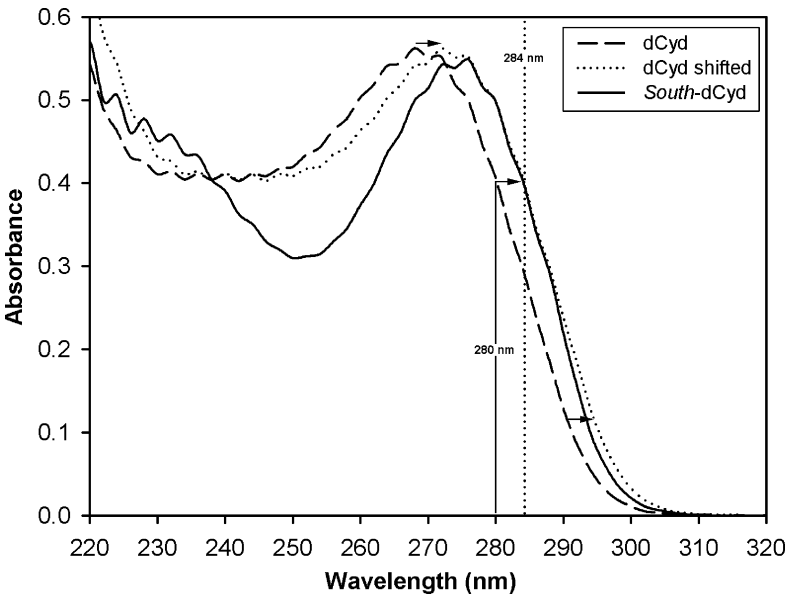
FIGURE 3S UV spectrum for 2'-deoxycytidine (dashed line) and South -dCyd (solid line). The UV spectrum of 2'-deoxycytidine, shifted by 4 nm is included for reference (dotted line).
